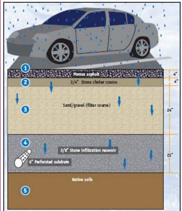
Cross-section of a Typical Porous Pavement System
